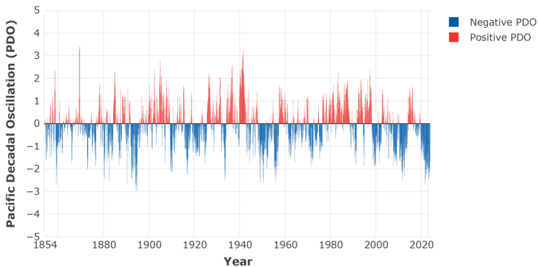
Figure 23. Pacific Decadal Oscillation from 1854–2023 with positive warm periods in red and negative cool periods in blue
