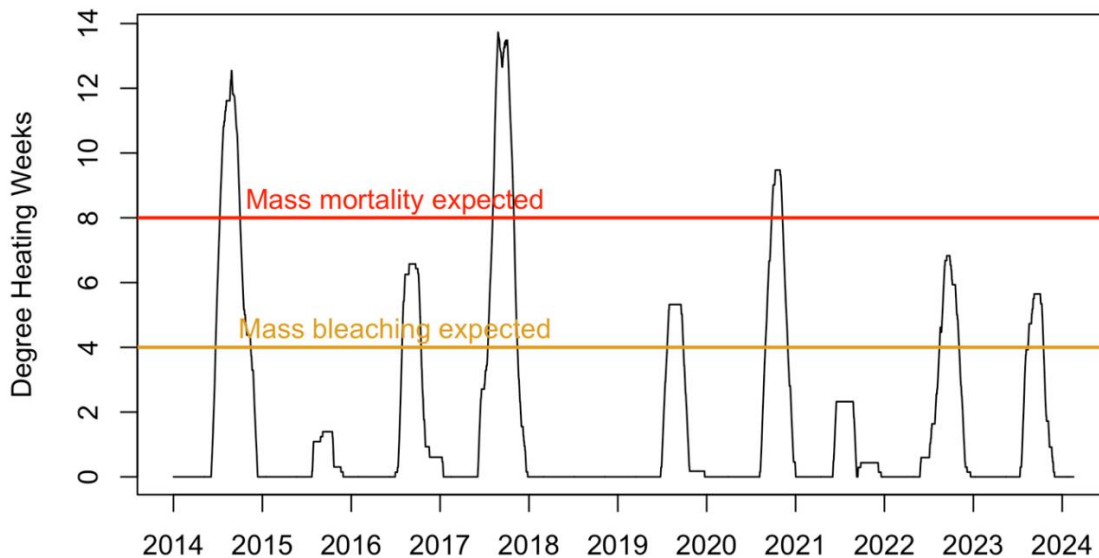
Figure 27. Coral Thermal Stress Exposure measured at CNMI Virtual Station 2014–2023 (Coral Reef Watch Degree Heating Weeks)
