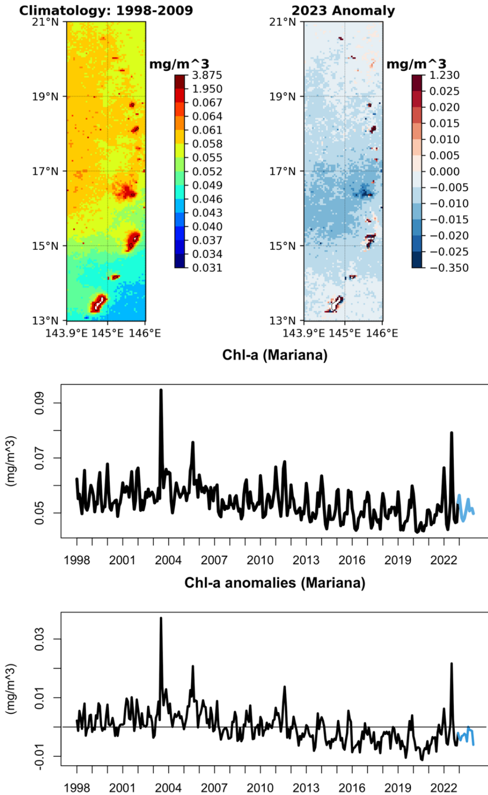
Figure 28. Chlorophyll- a (Chl-A) and Chl-A anomaly from 1998–2023
