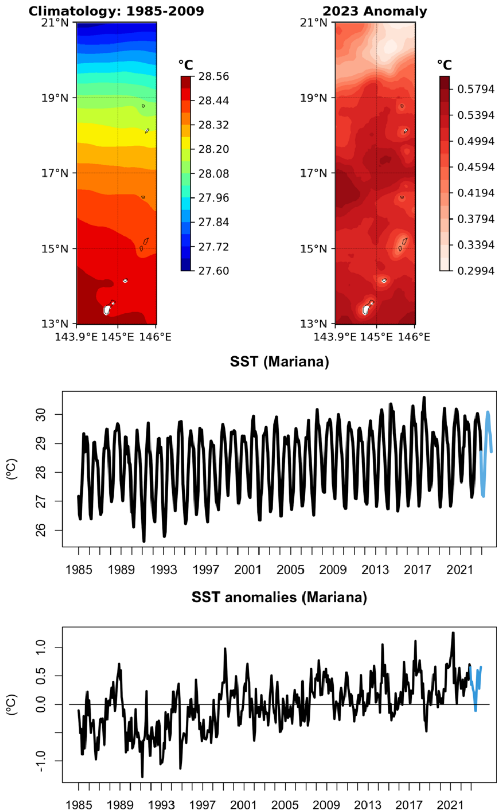
Figure 26. Sea surface temperature climatology and anomalies from 1985–2023
