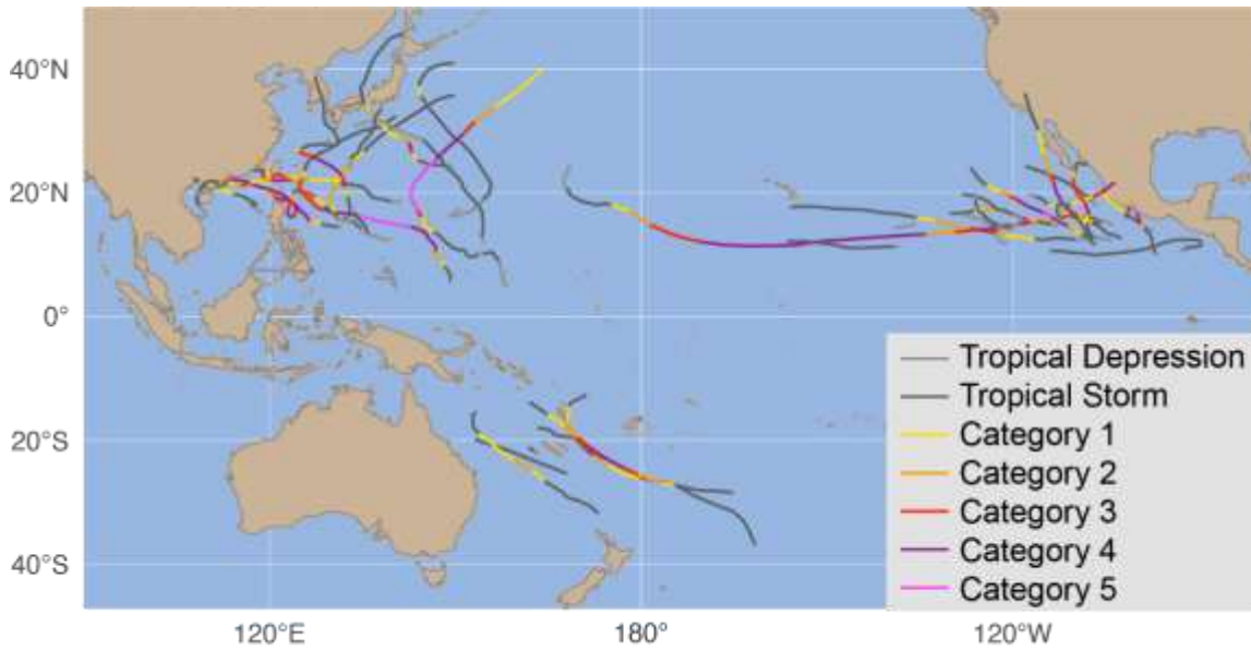
Figure 14. 2024 Pacific basin tropical cyclone tracks
