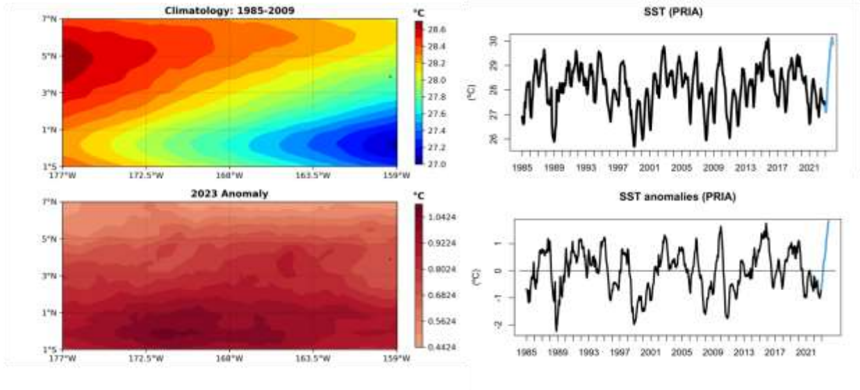
Figure 16. Sea surface temperature climatology and anomalies from the PRIA Grid
