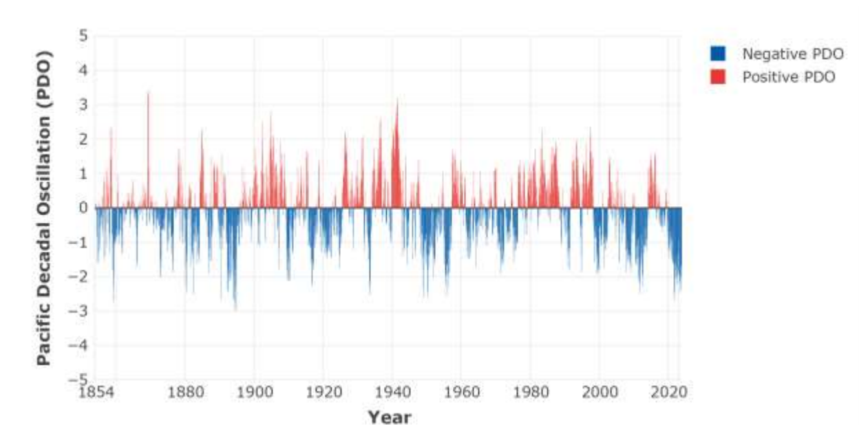
Figure 13. Pacific Decadal Oscillation from 1854–2023 with positive warm periods in red and negative cool periods in blue
