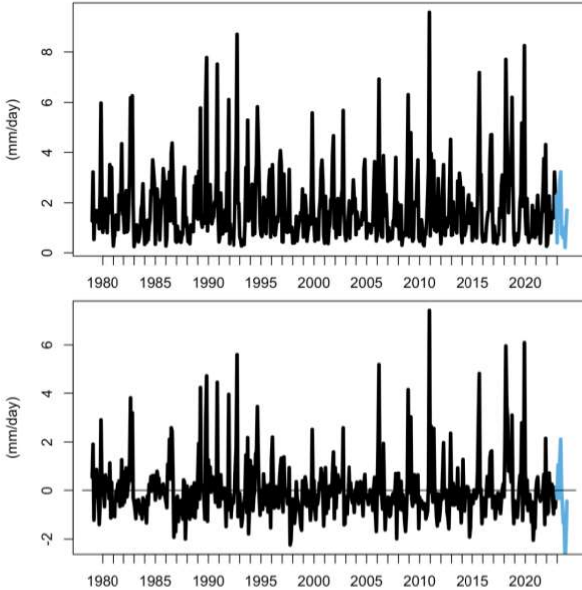
Figure 27. CMAP precipitation (top) and anomaly (bottom) across the Johnston Atoll Grid with 2023 values in blue
