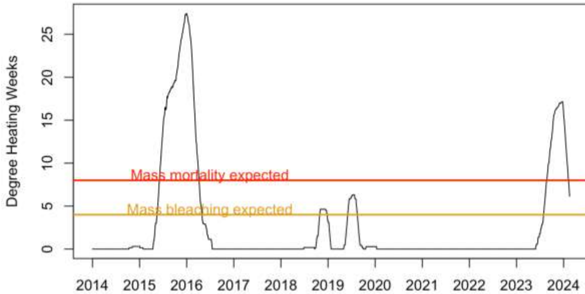
Figure 19. Coral Thermal Stress Exposure, Northern Line Islands Virtual Station 2014–2023 (Coral Reef Watch Degree Heating Weeks)
