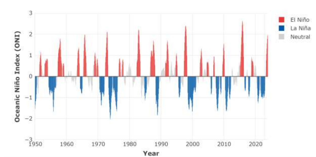
Figure 12. Oceanic Niño Index from 1950–2023 El Niño periods in red, La Niña periods in blue, and neutral periods in grey
