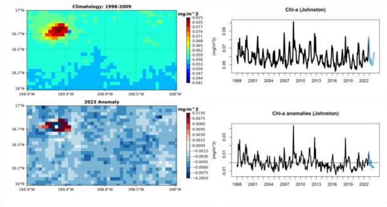
Figure 24. Chlorophyll-a and Chlorophyll-a Anomaly from the Johnston Atoll Grid
