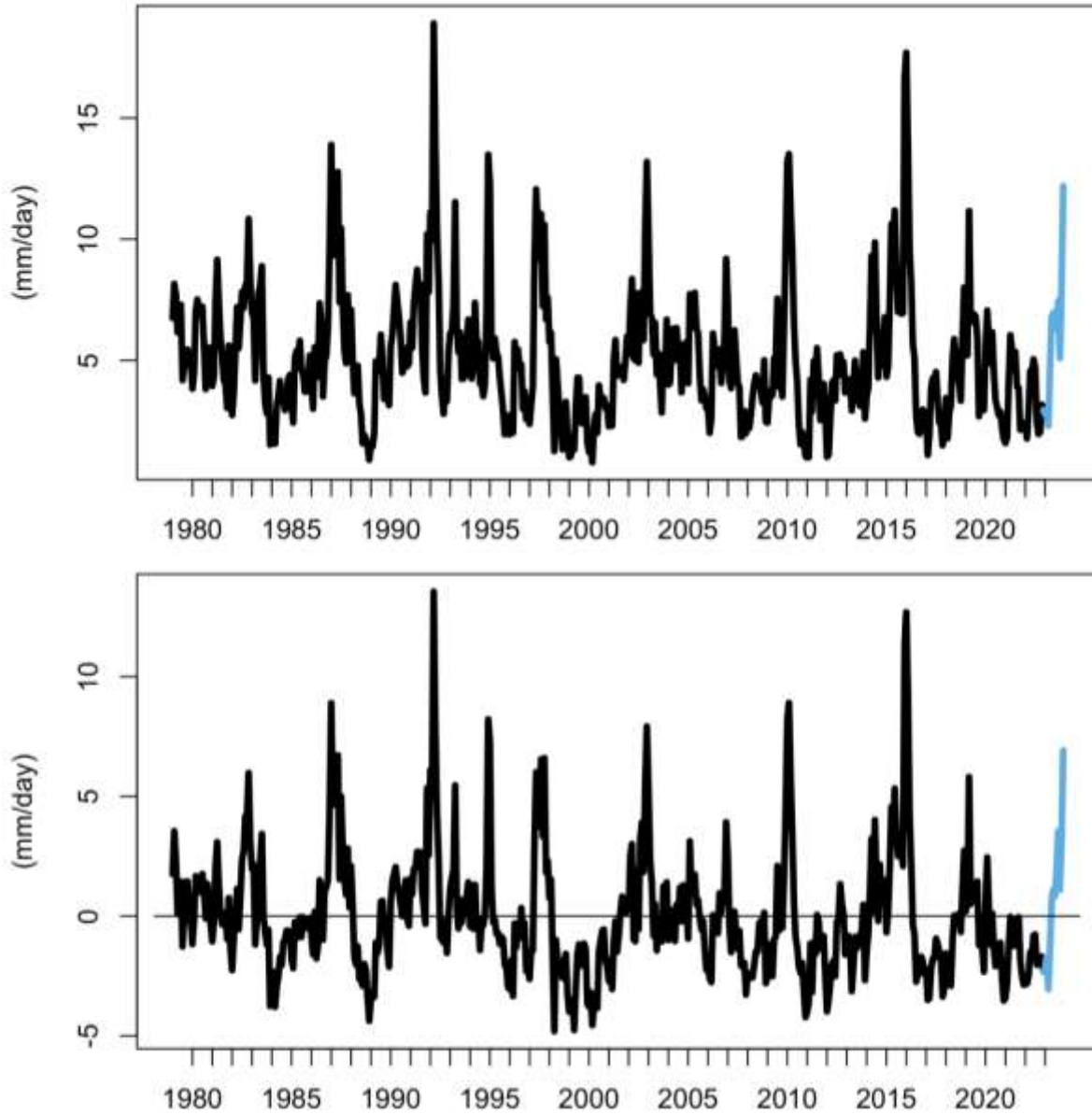
Figure 26. CMAP precipitation (top) and anomaly (bottom) across the PRIA Grid with 2023 values in blue
