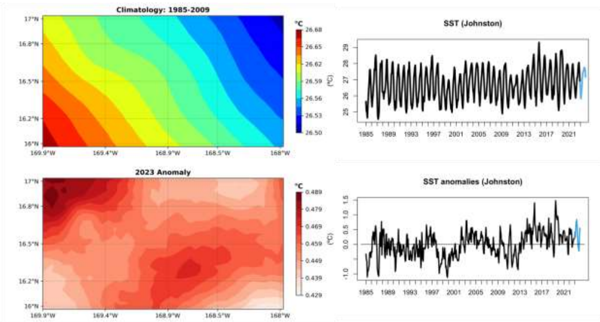
Figure 17. Sea surface temperature climatology and anomalies from Johnston Atoll Grid
