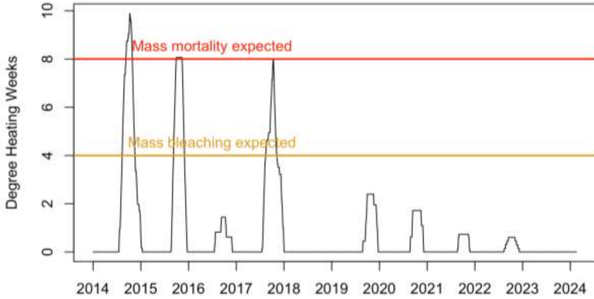
Figure 21. Coral Thermal Stress Exposure, Wake Atoll Virtual Station 2014–2023 (Coral Reef Watch Degree Heating Weeks)
