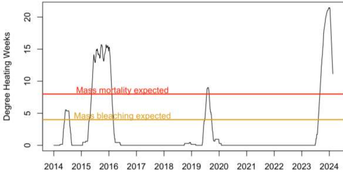
Figure 22. Coral Thermal Stress Exposure, Howland/Baker Virtual Station 2014–2023 (Coral Reef Watch Degree Heating Weeks)
