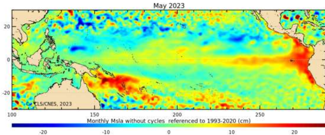
Figure 29a. Sea surface height and anomaly across the Pacific Ocean
