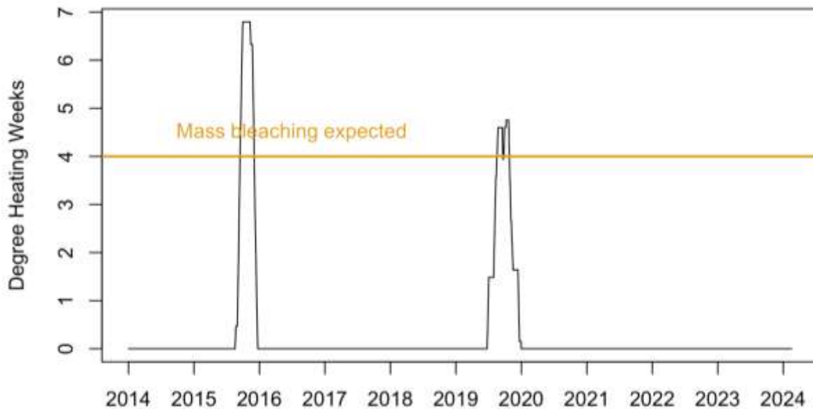
Figure 20. Coral Thermal Stress Exposure, Johnston Atoll Virtual Station 2014–2023 (Coral Reef Watch Degree Heating Weeks)
