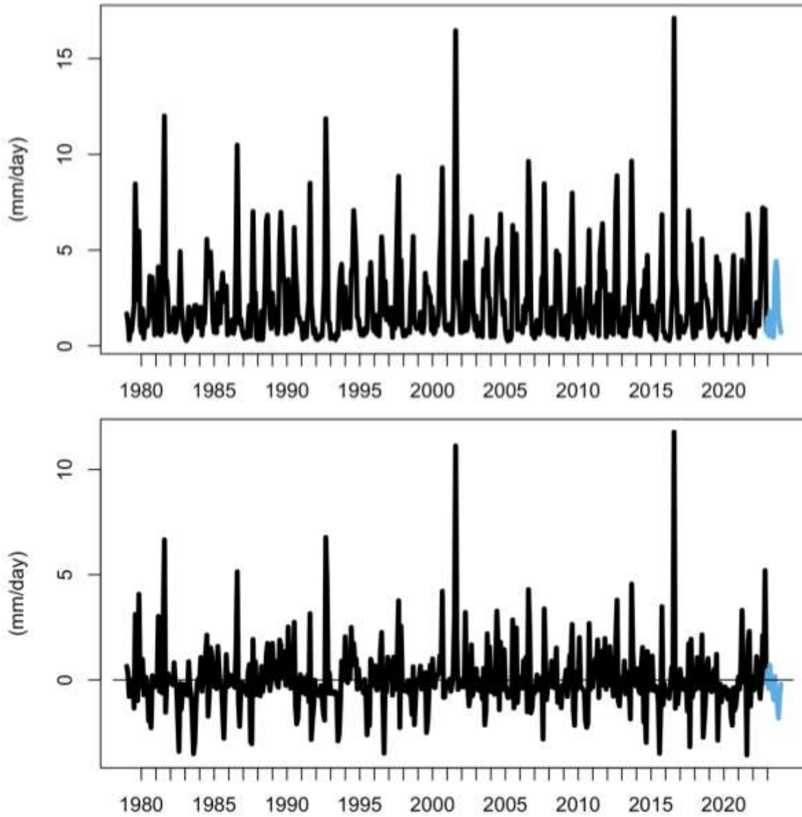
Figure 28. CMAP precipitation (top) and anomaly (bottom) across the Wake Atoll Grid with 2023 values in blue
