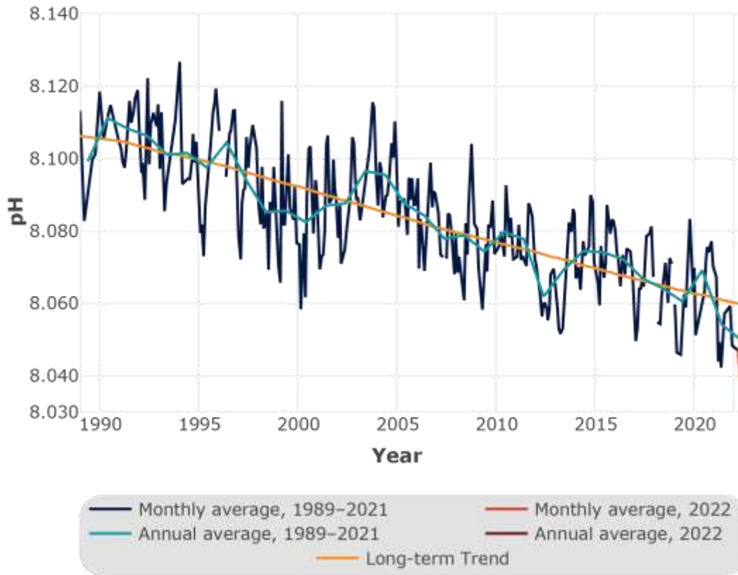
Figure 11. Time series and long-term trend of oceanic pH measured at Station ALOHA
