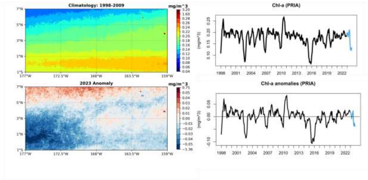
Figure 23. Chlorophyll-a and Chlorophyll-a Anomaly from the PRIA Grid
