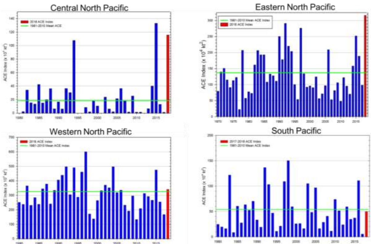
Figure 33. 2018 Accumulated Cyclone Energy (ACE) Index by region
