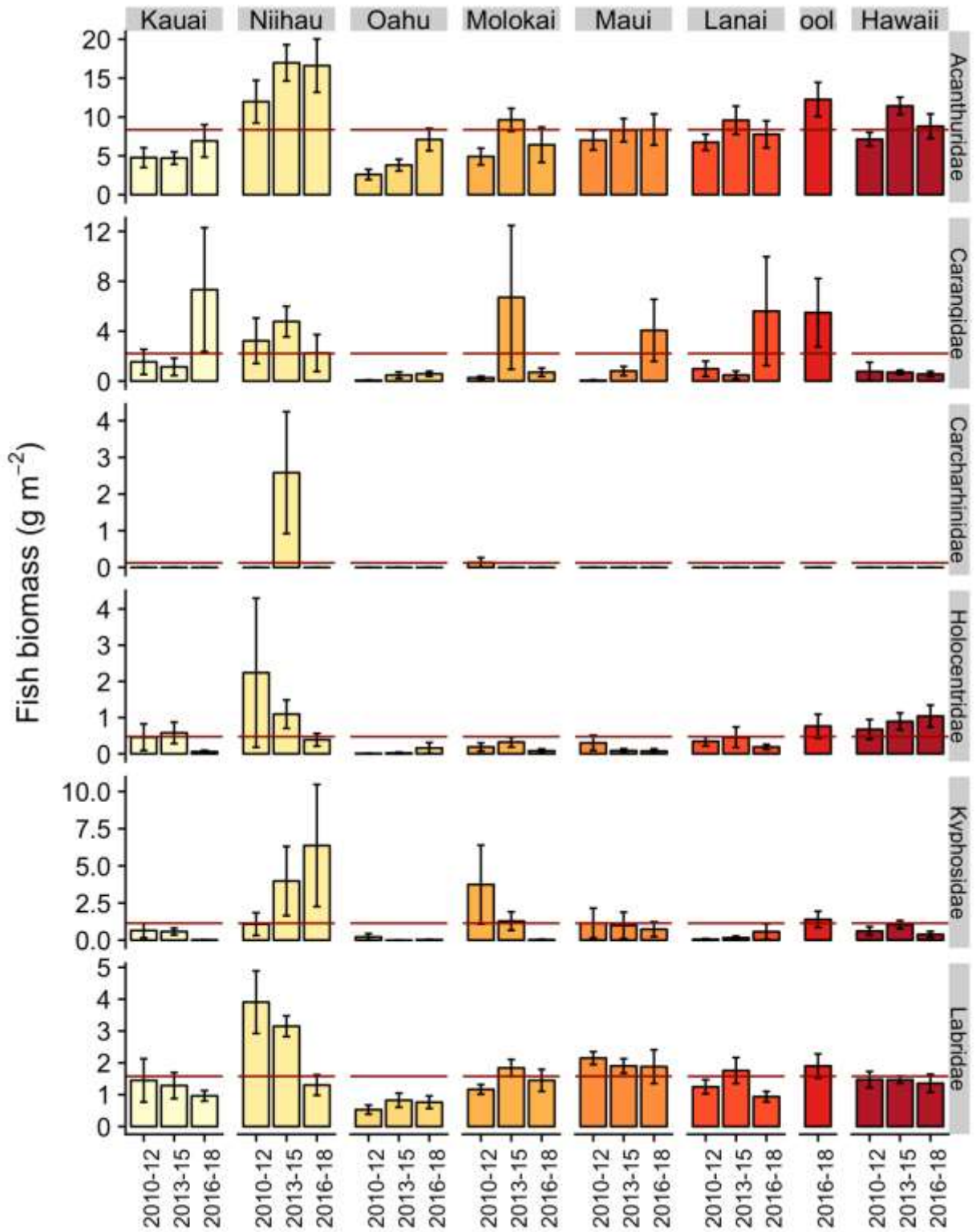
Figure 7. Mean fish biomass (g/m 2 ± standard error) of MHI CREMUS from the years 2010-2018 with mean estimates overlaid in red; figure continued on next page
