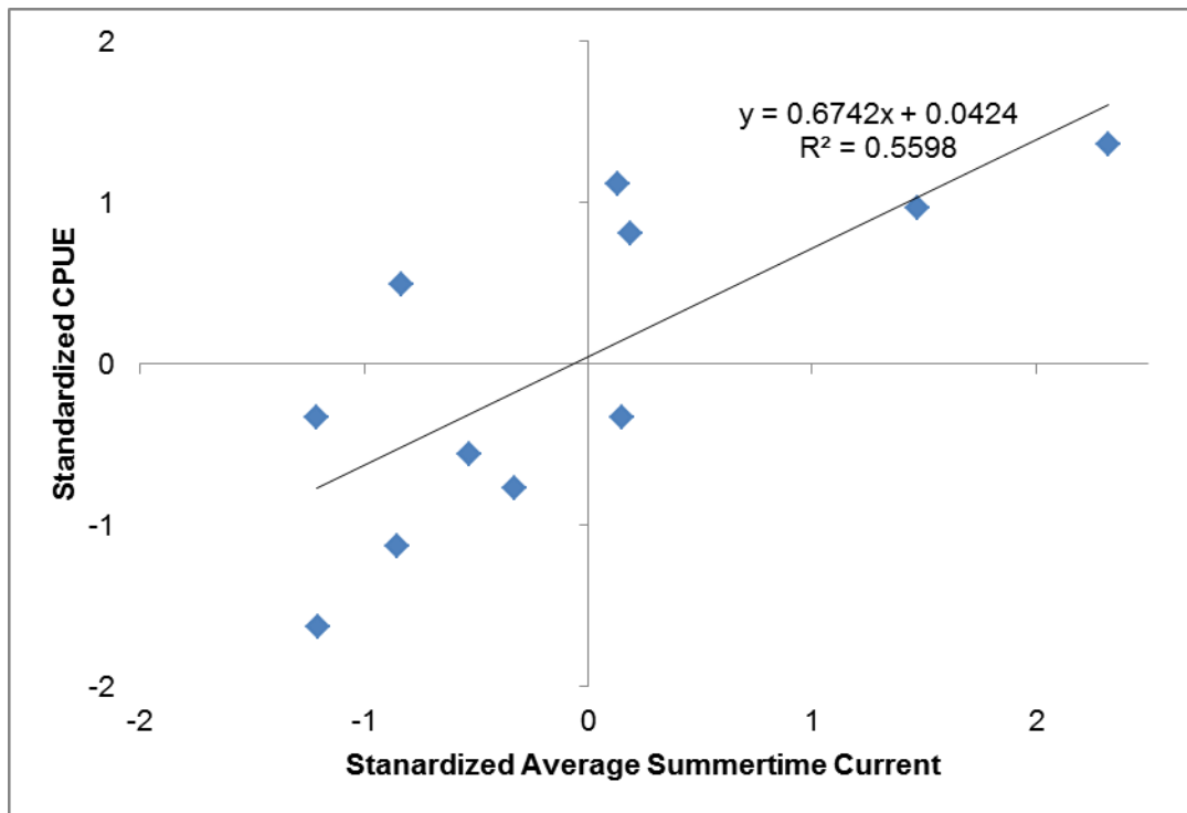
Figure 52. Standardized CPUE for uku from the MHI from 2002-2012 plotted against standardized average summertime zonal current with a phase lag of two years
