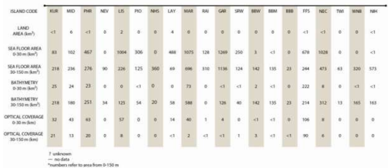
Figure 42. NWHI land and seafloor with primary data coverage
