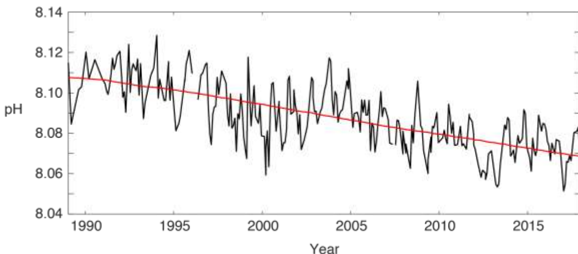
Figure 28. Oceanic pH (black) and its trend (red) at Station ALOHA from 1989 – 2017
