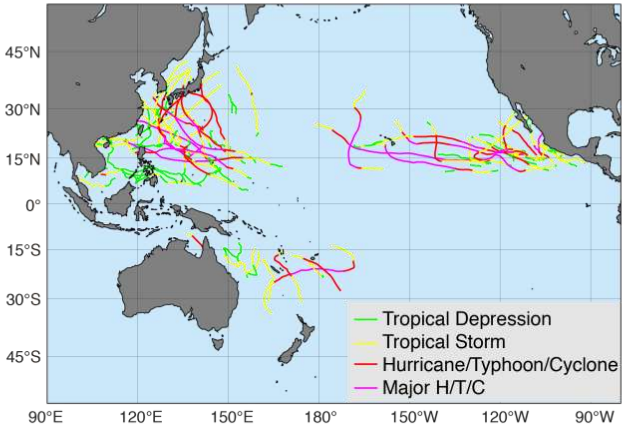
Figure 31. 2018 Pacific basin tropical cyclone tracks
