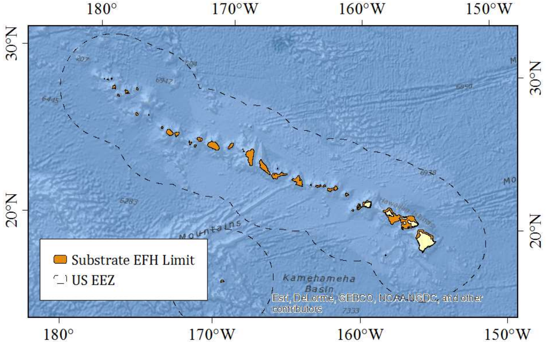
Figure 40. Substrate EFH limit of 700 m isobath around the Hawaiian Archipelago (from GMRT; Ryan et al., 2009)
