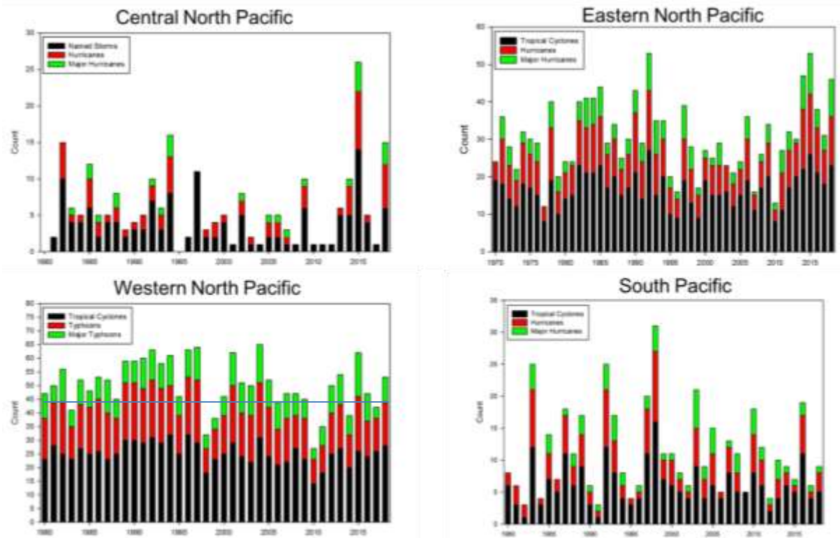
Figure 32. 2018 tropical storm totals by region
