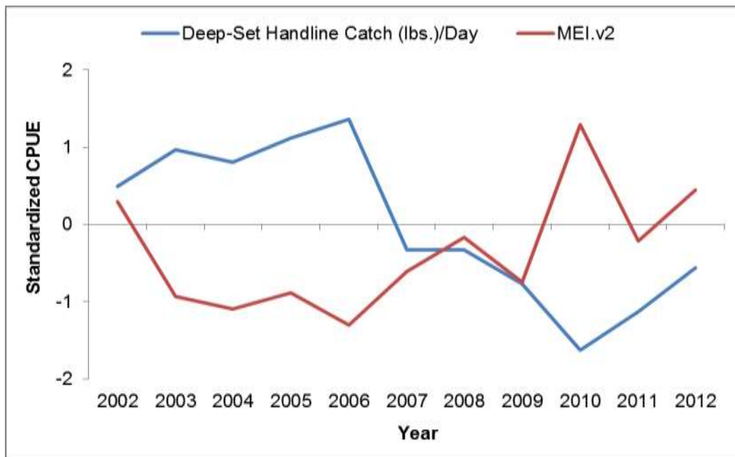
Figure 48. Comparison of standardized MHI Deep-Set Handline CPUE and MEI.v2 with a phase lag of two years from 2002-2012 ( r = -0.729 )
