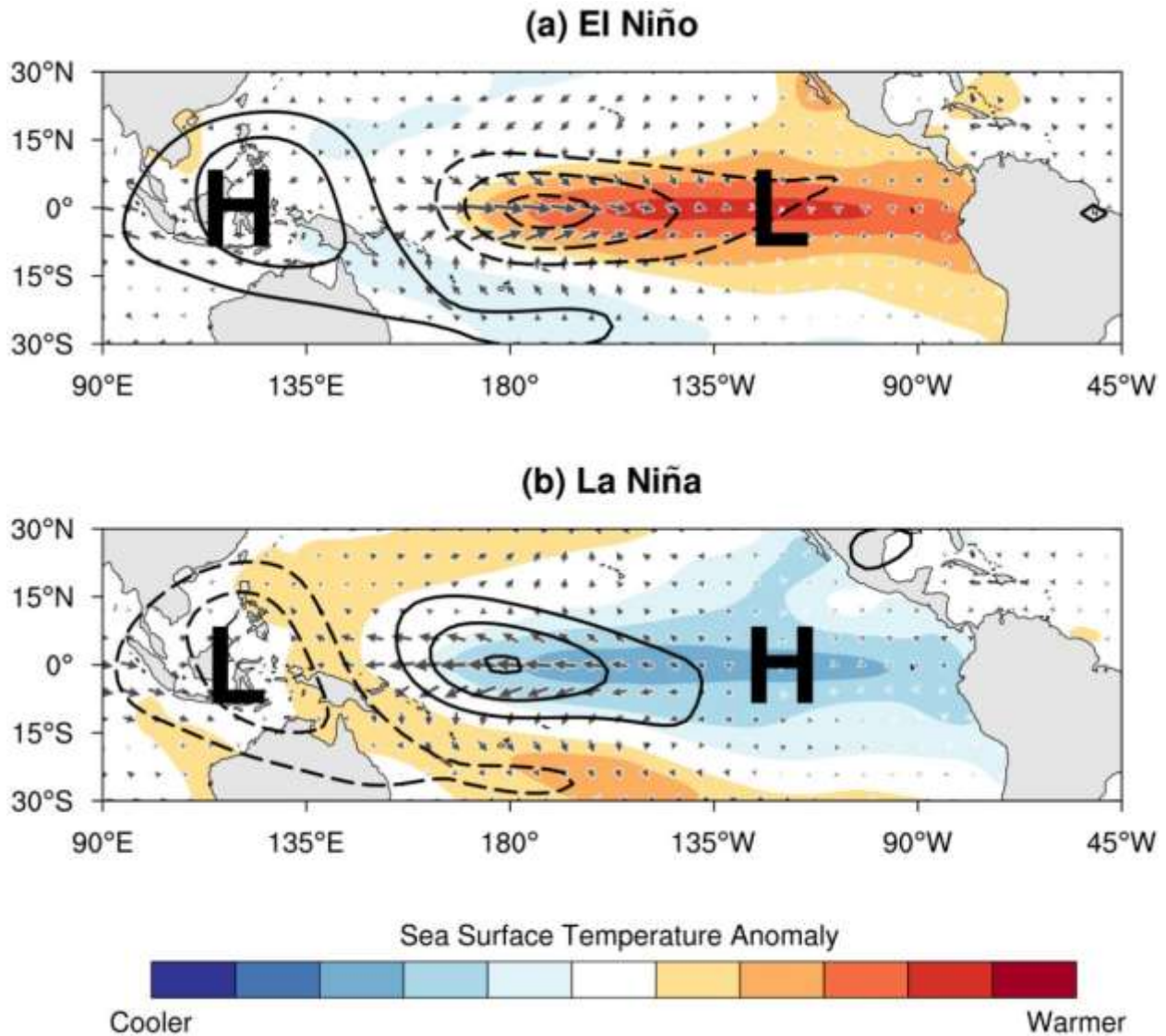
Figure 46. Diagram showing the physical mechanisms by which the SST (shaded), OLR (contours), surface zonal and meridional winds (vectors), and sea level pressure (represented by “H” and “L”) determine the wintertime Multivariate ENSO Index (MEI) during (a) El Niño and (b) La Niña events” (from NOAA 2019)
