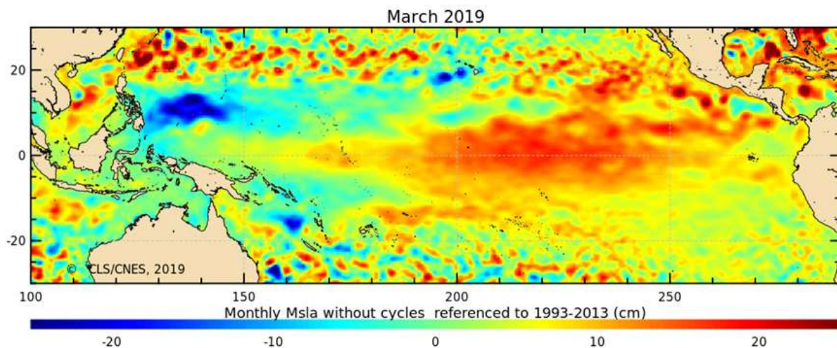
Figure 38a. Sea surface height and anomaly
