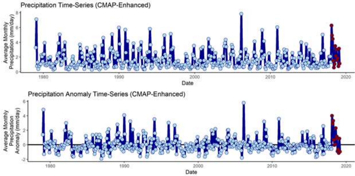
Figure 37. CMAP precipitation across the MHI Grid with 2018 values in red
