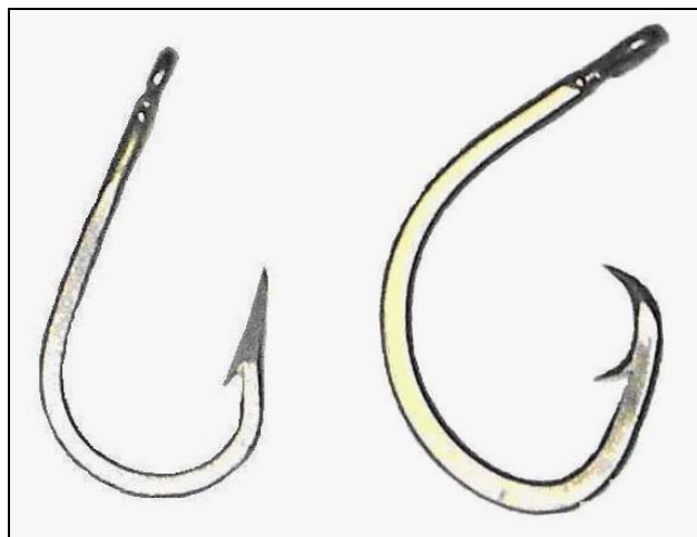
Fig. 1. 9/0 J hook manufactured by Mustad (left) 4.0 cm narrowest width, and 10 degree offset 18/0 circle hook manufactured by Lingren-Pitman 4.9 cm narrowest width (photo E. Gilman). Hooks are oriented so that the narrowest width is horizontal. Differences in hook designs other than narrowest width (i.e. orientation of point, length, gape, bite) and materials may also be important variables affecting sea turtle capture rates and position of hooking.
